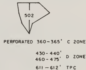
Figure 11- STIFF DIAGRAMS OF GROUND WATERS - NIPOMO MESA
