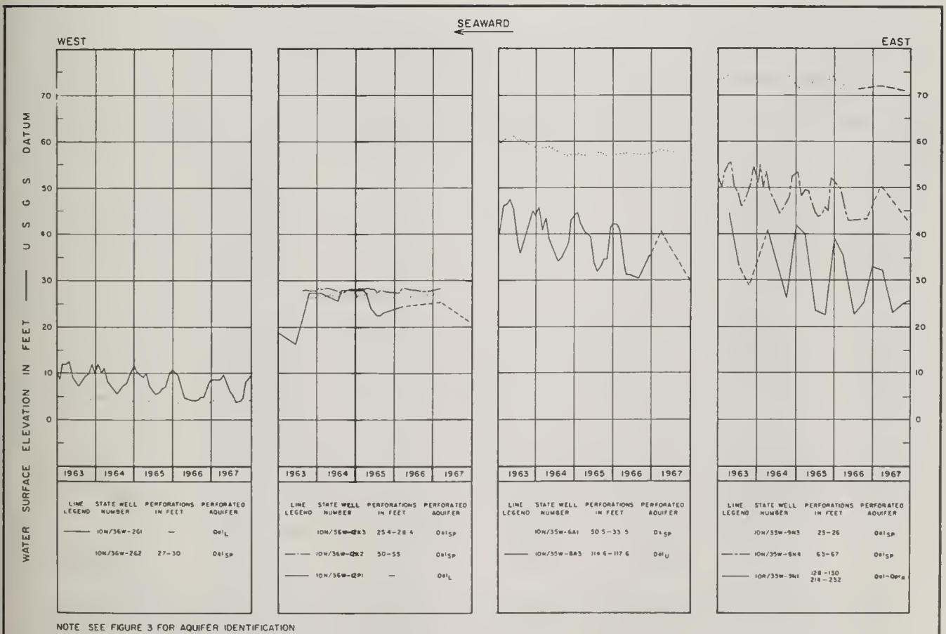
Figure 6. HEAD RELATIONSHIP BETWEEN SEMIPERCHED AND CONFINED GROUND WATERS - SANTA MARIA HYDROLOGIC SUBUNIT
