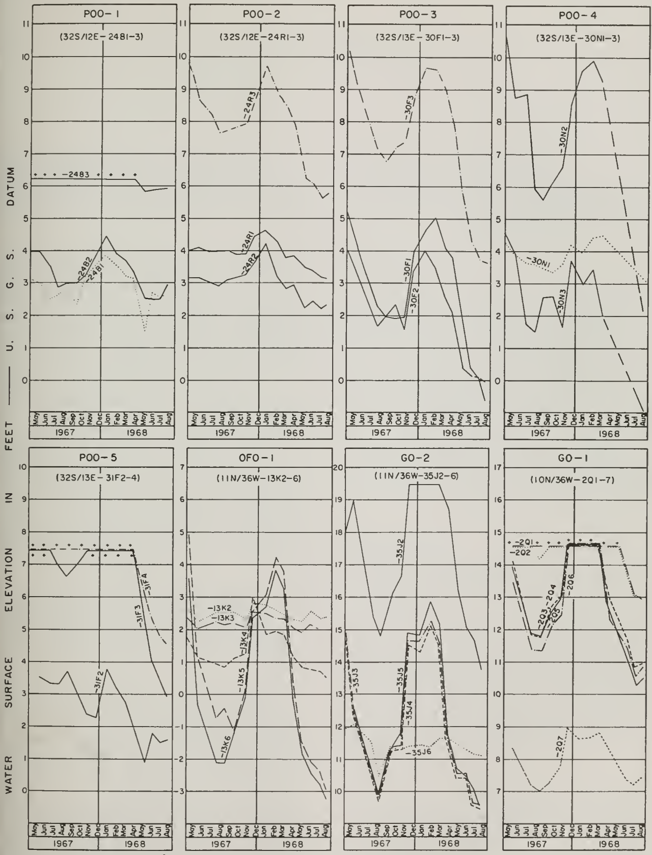
Figure 7. HYDROGRAPHS OF WATER LEVEL IN OBSERVATION WELLS
