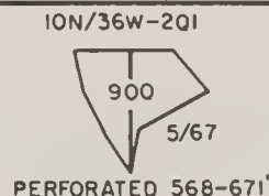
Figure 12. STIFF DIAGRAMS OF GROUND WATERS—SANTA MARIA HYDROLOGIC SUBUNIT
